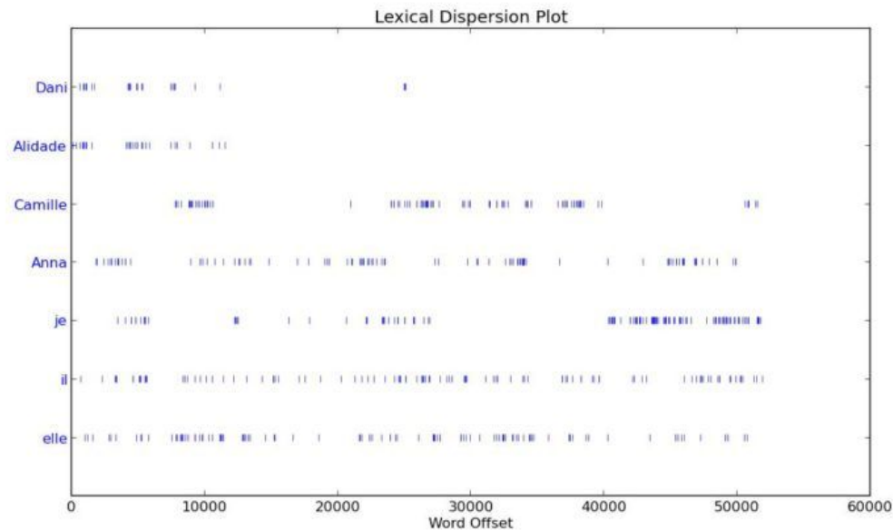
Figure 3 : Dispersion Plot
